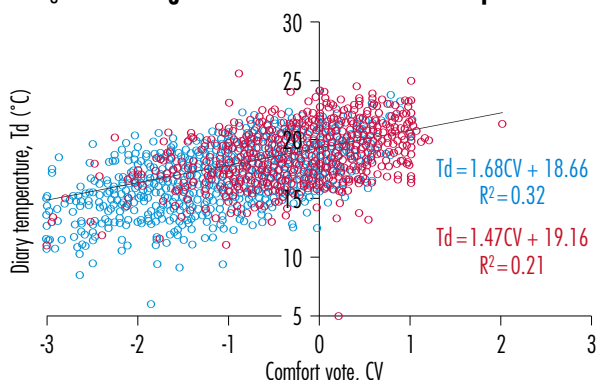
Figure 17: Living room thermal comfort and temperature
